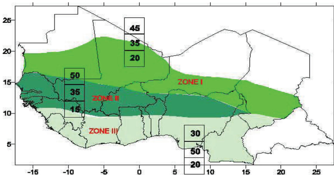
Figure 1. PRESAO-11 RCOF consensus forecast issued 21 May 2008
