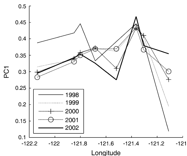
Fig. 8 PC1 for each year from 1998 to 2002 taken individually for the stations that had data for that time period (2, 3, 9, 10, 13, 14, 15, and 16). The x -axis represents longitude and the y -axis represents PC1
