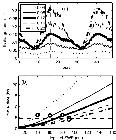
Figure 16. (a) Discharge/meltwater flux versus time as a function of melt rate (cm hr -1 ). The line plotted for each melt rate is the sum of output from 16 snow depths (25–400 cm), where small spikes indicate the individual peaks. Notice that as the melt rate increases, the individual spikes become closer together, resulting in a longer period of smooth decline in the daily cycle. The time of diurnal peak for the average remains close to 1630 for all melt rates, in spite of the shift to earlier peak timing experienced by each individual snow depth. (b) The travel time spent in the snowpack as a function of snow depth for each of the five melt rates. The circles identify the average travel time for all 16 snow depths, including the effects of aliasing (i.e., a delay of 28 hours would contribute to an average delay of 4 hours). The depth at which the shock front occurs can be identified by the kink in each line, where the velocity slows and travel time increases more rapidly with depth.
